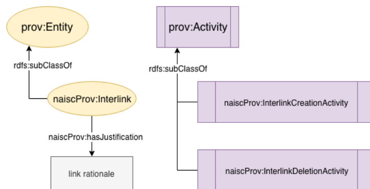
Figure 2: NaiscProv PROV-O Extension
