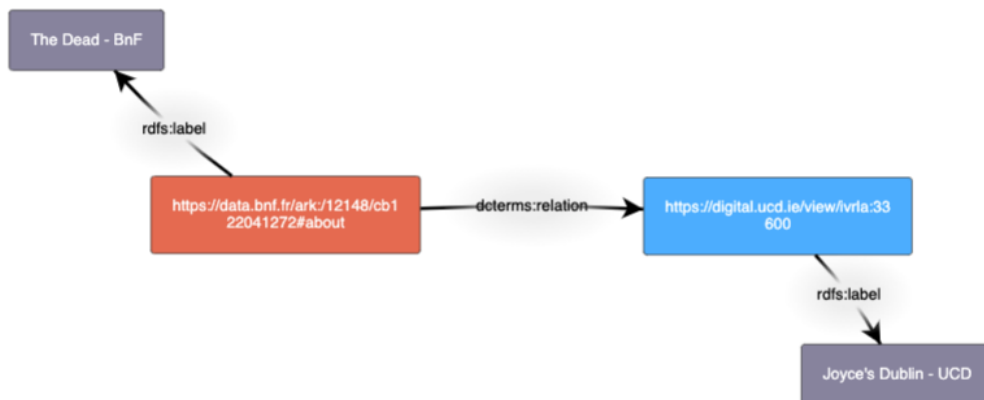
Figure 8: Interlink Graph Visualisation (created using GoJS xv )
